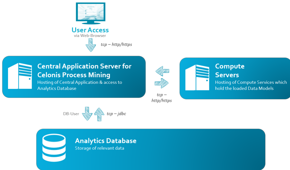
Figure 2: Multi-server deployment
